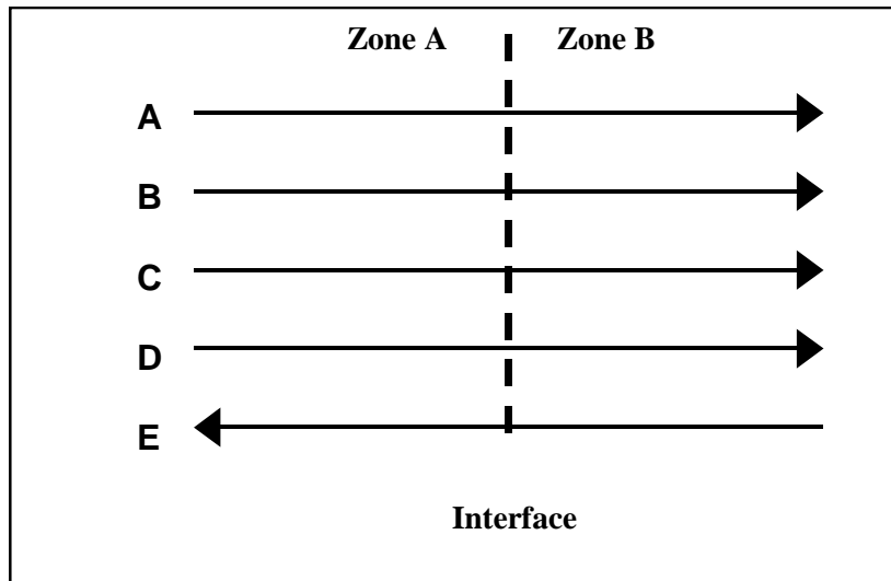
Figure 4-3: Transaction Example
